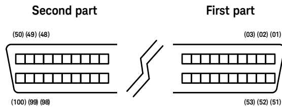
Figure 2-2 Connector in horizontal view
