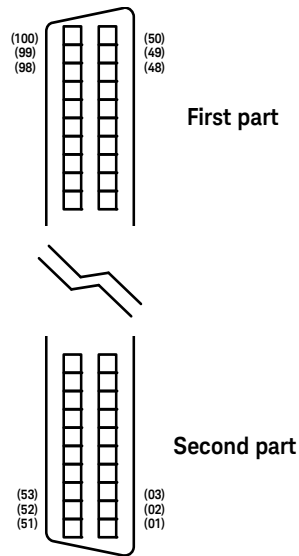
Figure 2-1 Connector in vertical view
