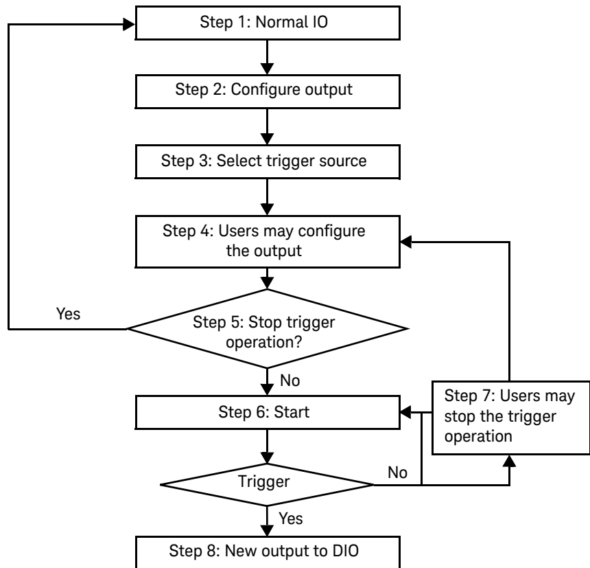
Figure 3-7 Flowchart for trigger function operation
