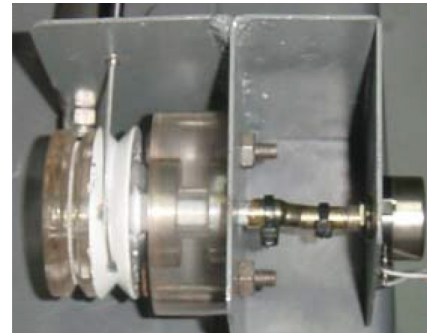
Figure 5. TPS pot (right) and throttle linkage (left)
