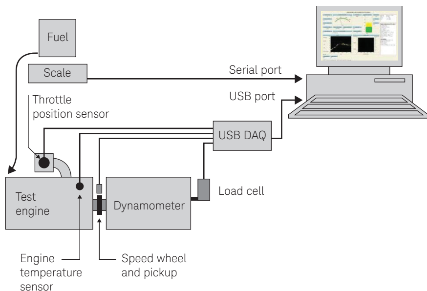
Figure 1. Schematic overview of test system
