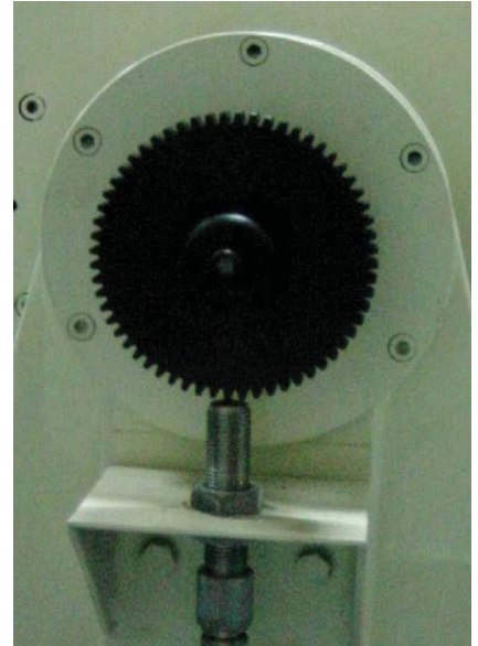
Figure 4. Speed wheel (top) and pickup (below)
