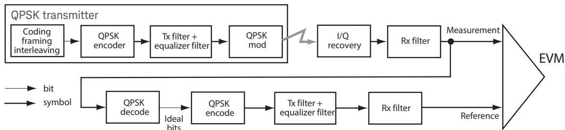
Figure 10. Process to calculate EVM for a QPSK signal.
