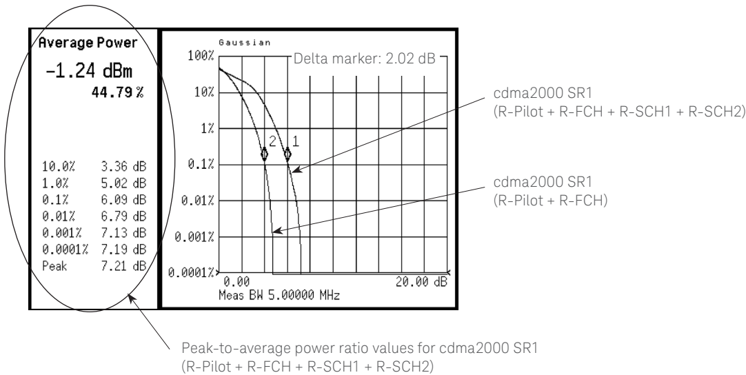
Figure 6. CCDF curves for two cdma2000 SR1 reverse link signals with different channel configurations.
