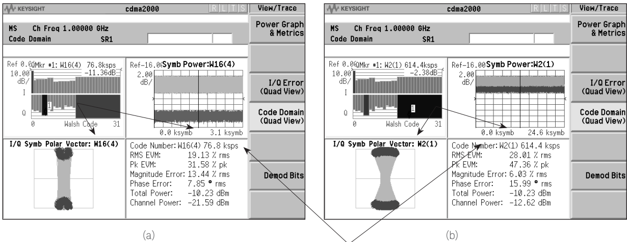
Impairment causes higher symbol EVM in high data rate channel
