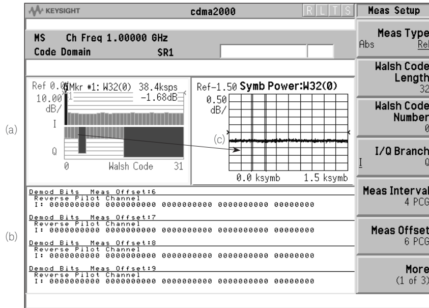
Figure 24. (a) cdma2000 code domain power measurement (bit-reverse display) for a signal with R-Pilot, an R-FCH ( W_4^{16} at -12.77 dB), and an R-SCH1 ( W_1^2 at -3.77 dB). (b) Demodulated bits for the R-Pilot. (c) Symbol power versus time for the R-Pilot.
