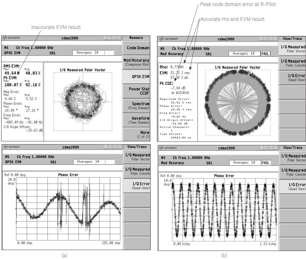
Figure 15. cdma2000 R-Pilot signal with very high LO instability. (a) Vector diagram and phase error versus time for QPSK EVM. (b) Vector diagram and phase error versus time for composite EVM (provided with composite rho measurement).
