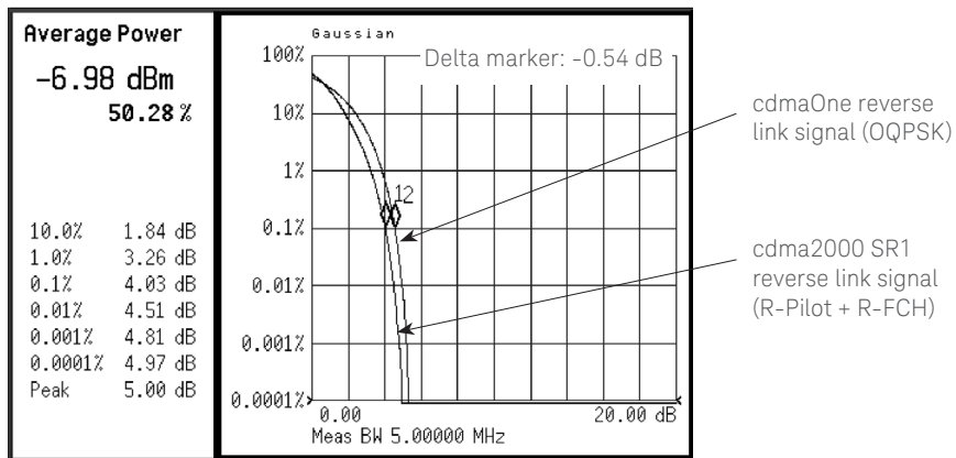
Figure 7. CCDF comparison between cdmaOne and cdma2000 reverse link signals.
