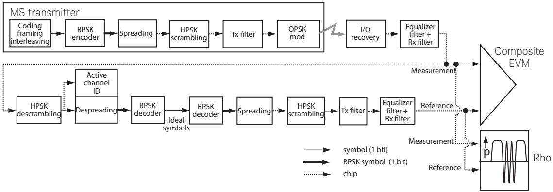
Figure 13. Process to calculate composite rho and composite EVM for a cdma2000 reverse link signal.
