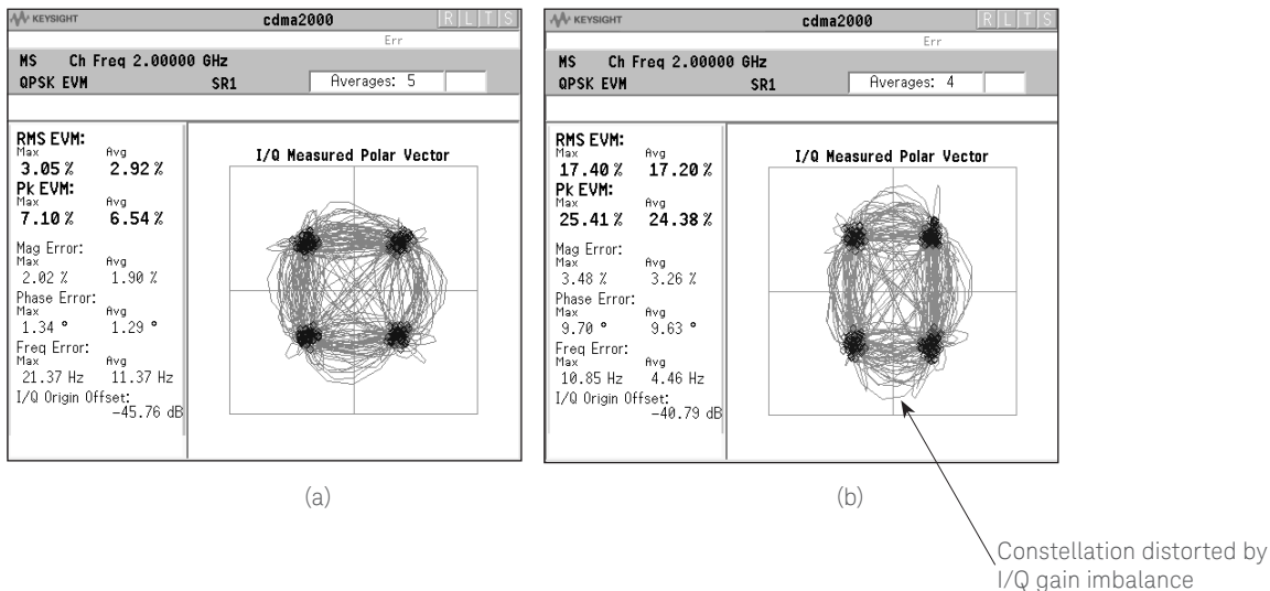
Figure 12. QPSK EVM on a cdma2000 reverse link signal with a single R-Pilot channel, (a) without any impairments, and (b) with an I/Q gain impairment.
