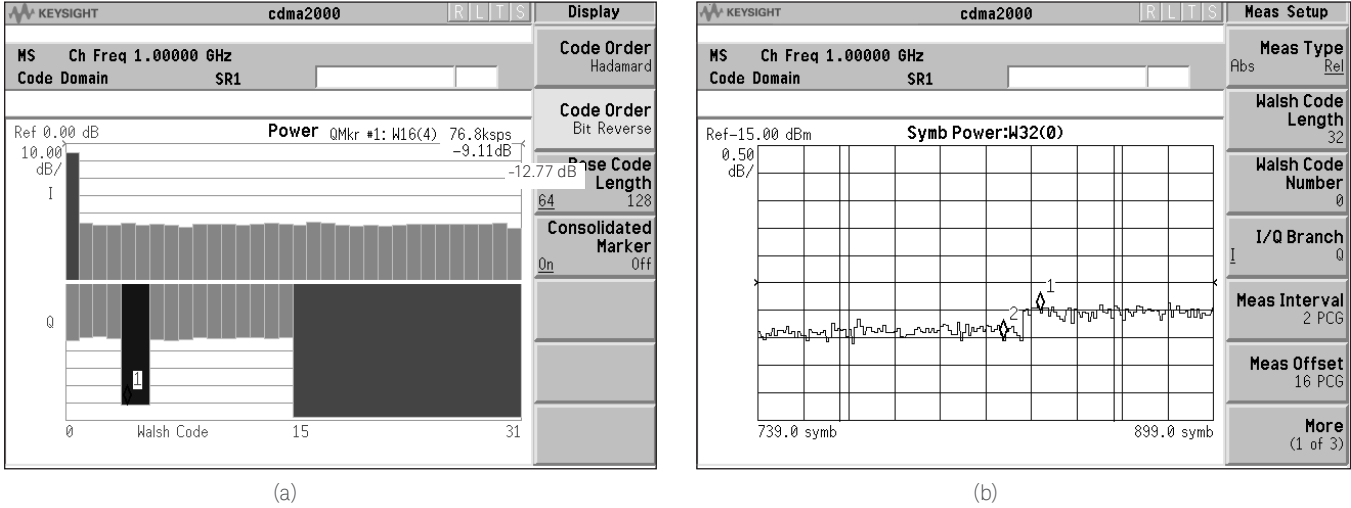
Figure 22. (a) cdma2000 code domain power measurement (bit reverse display) for a signal with an R-Pilot, an R-FCH ( W_4^{16} at -12.77 dB), and an R-SCH1 ( W_1^2 at -3.77 dB). (b) Symbol power versus time for the R-FCH.
