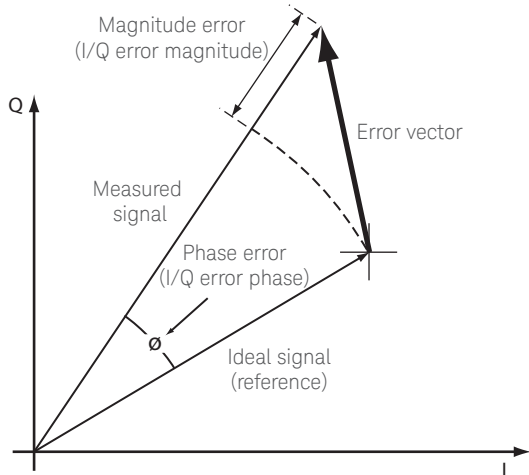
Figure 9. Error vector and related parameters.
