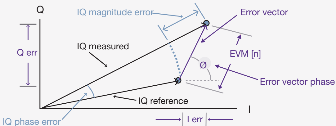
Figure 1. Understanding the EVM calculation
