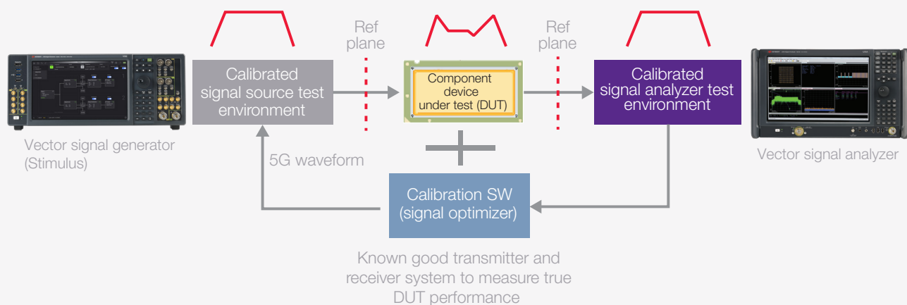
Figure 2. 5G R&D Test Bed with 5G NR-ready hardware and software, including signal optimizer calibration software
