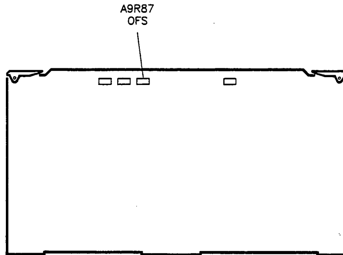
Figure 3-15. Amplifier Detector Offset Adjustment Location
