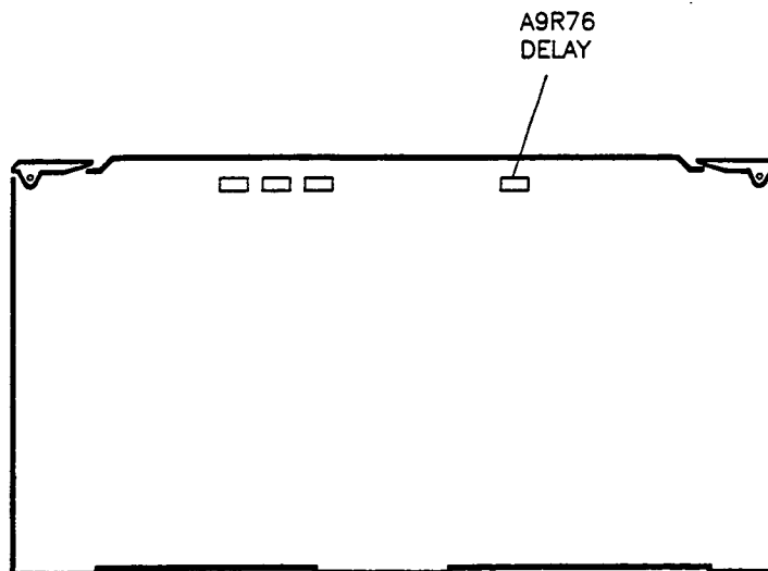
Figure 3-36. Pulse Delay Adjustment Location
