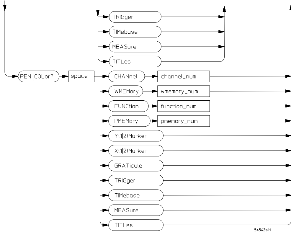
Hardcopy Subsystem Commands Syntax Diagram (continued)
